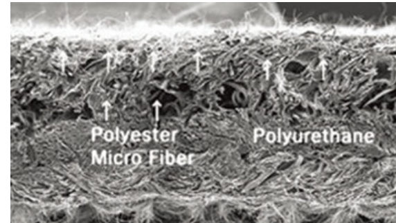
Cross Section of LASEDE®
